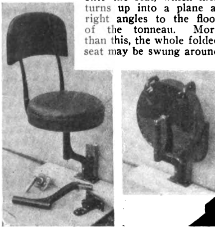
READY FOR USE. FOLDED UP. HILL FOLDING TONNEAU SEAT.
